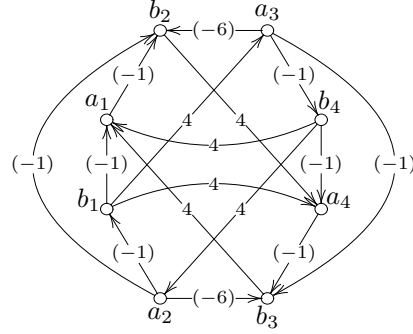
Figure 2: The inequalities and directed graph H for the graph from Figure 1.
