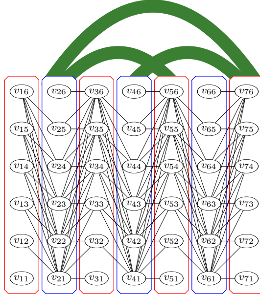
Figure 4: The Z -grid Z_{n,m} with n = 7 columns and m = 6 rows, where in addition (indicated in green) every vertex in the i -th column with an even i is adjacent to every vertex in the j -th column with an odd j \geq i + 3 .
